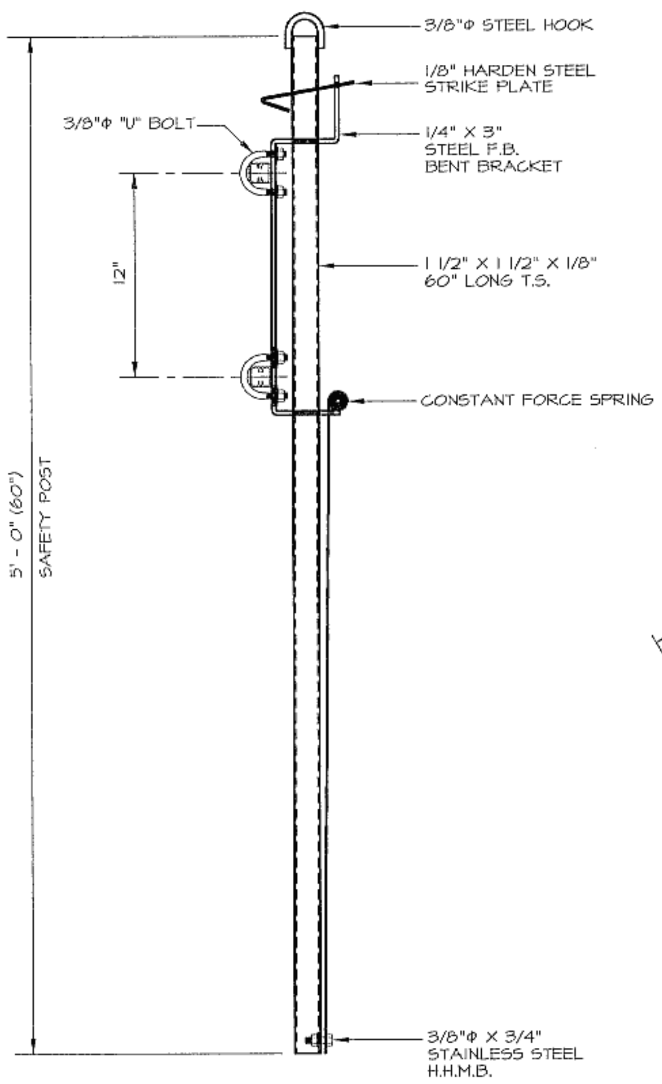
SAFETY POST 1" = 1' - 0"
