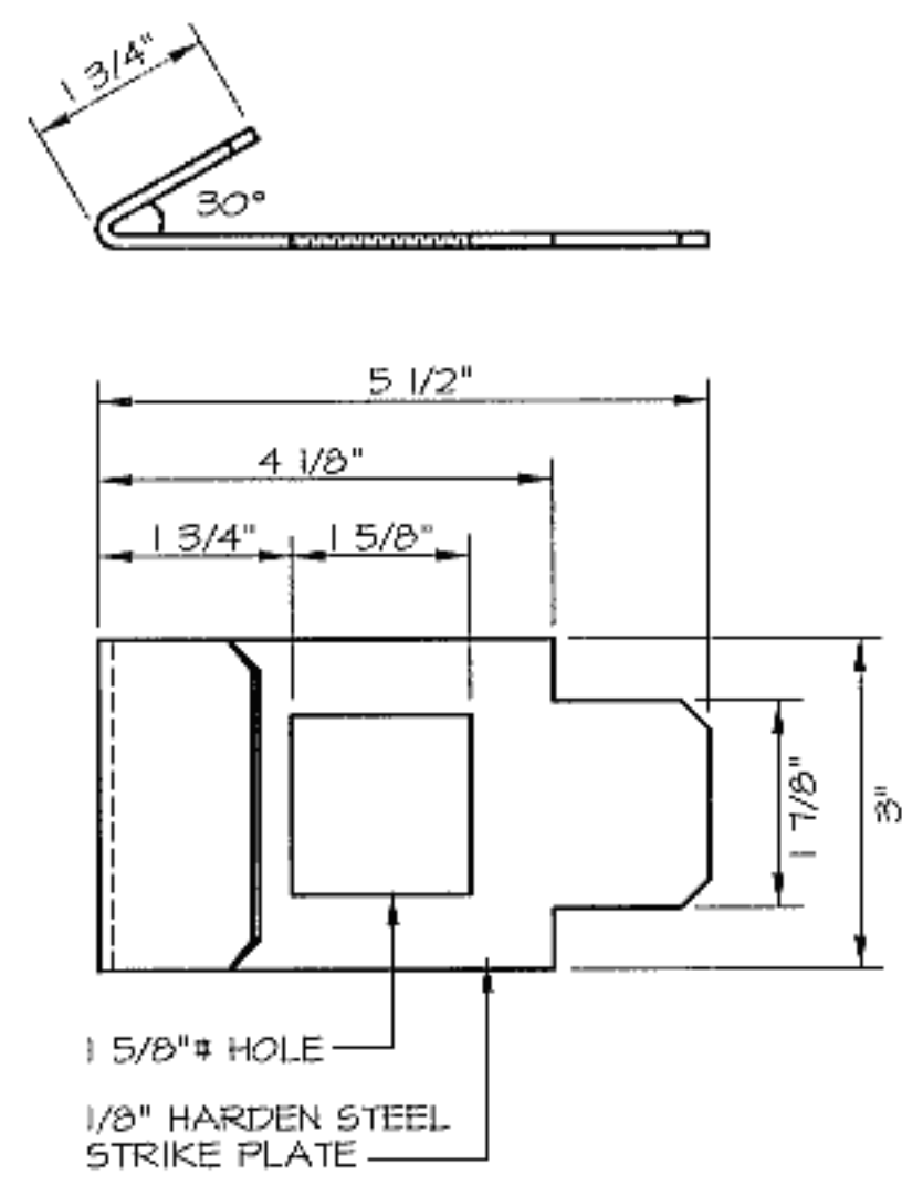
STRIKE PLATE 3" = 1' - 0"
