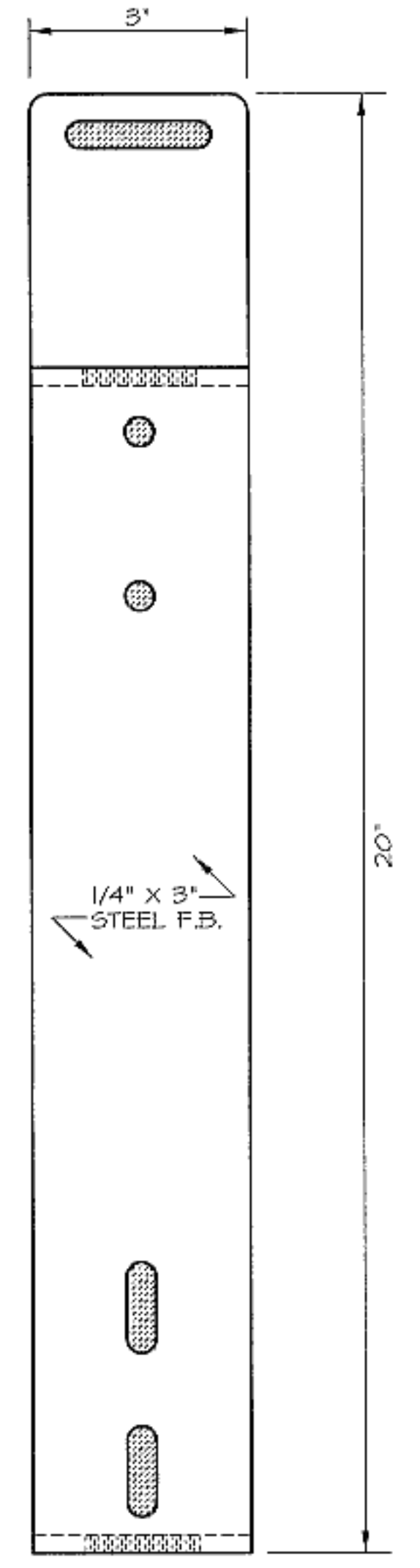
BRACKET 3" = 1' - 0" FRONT VIEW
