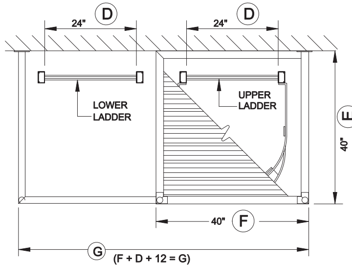
A PLATFORM PLAN 3/8" = 1' - 0"
