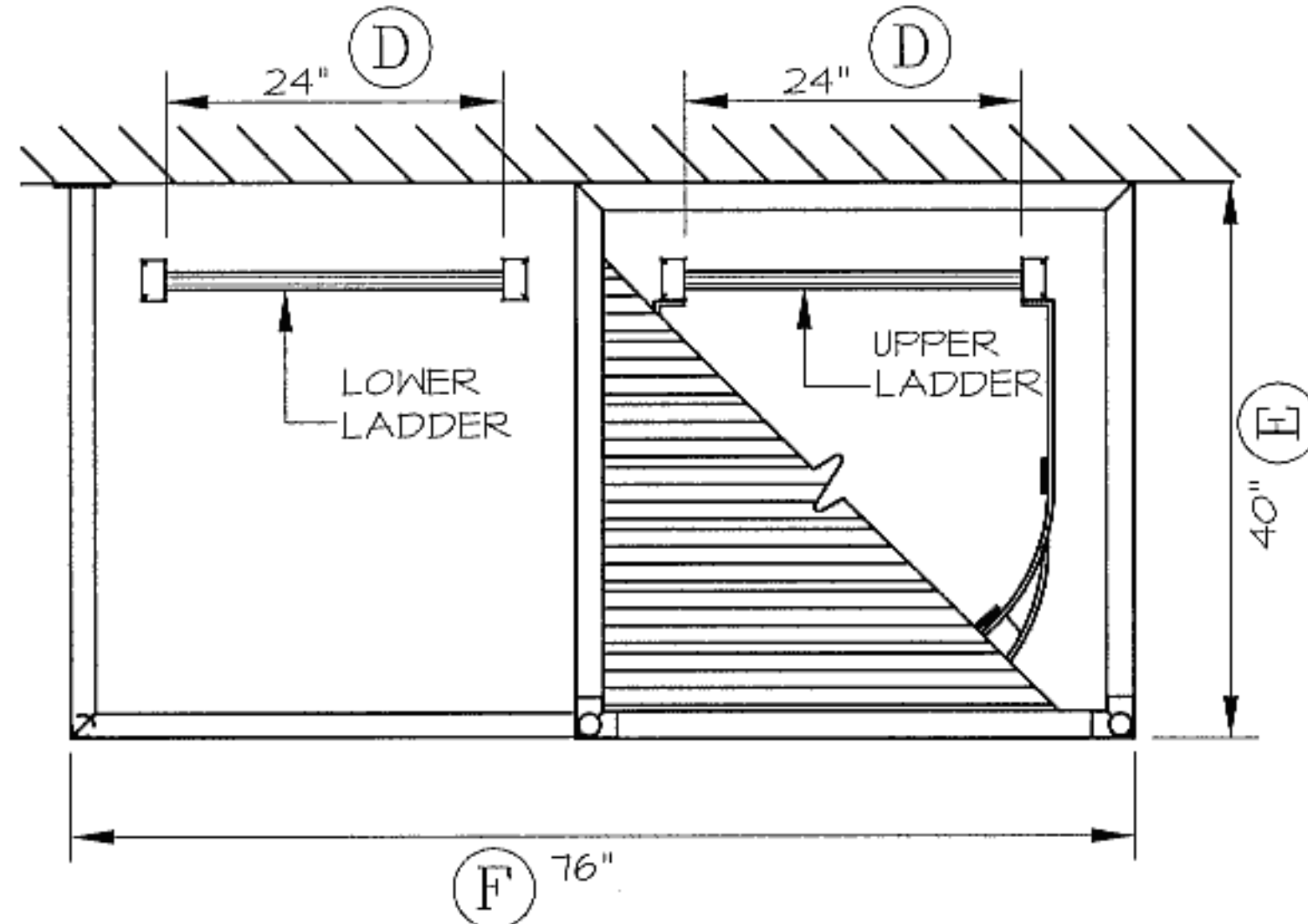
A PLATFORM PLAN 3/8" = 1' - 0"
