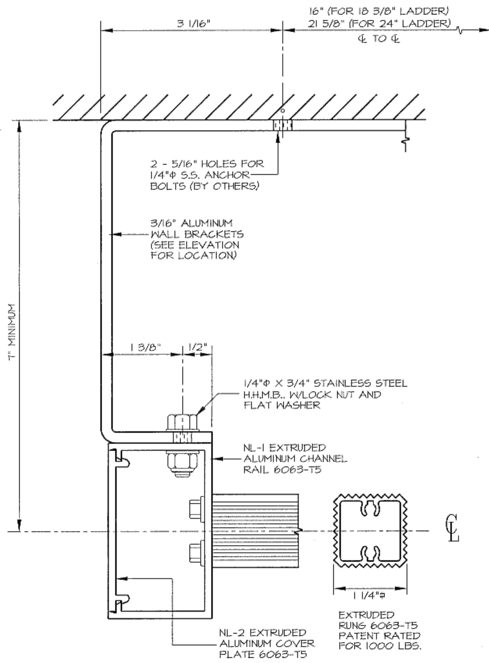
ALTERNATE BRACKET 1/2 FULL SCALE
