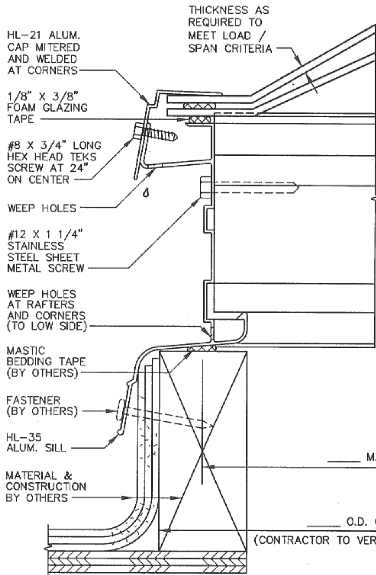
① CURB MOUNTED SILL 1/2 FULL SCALE
