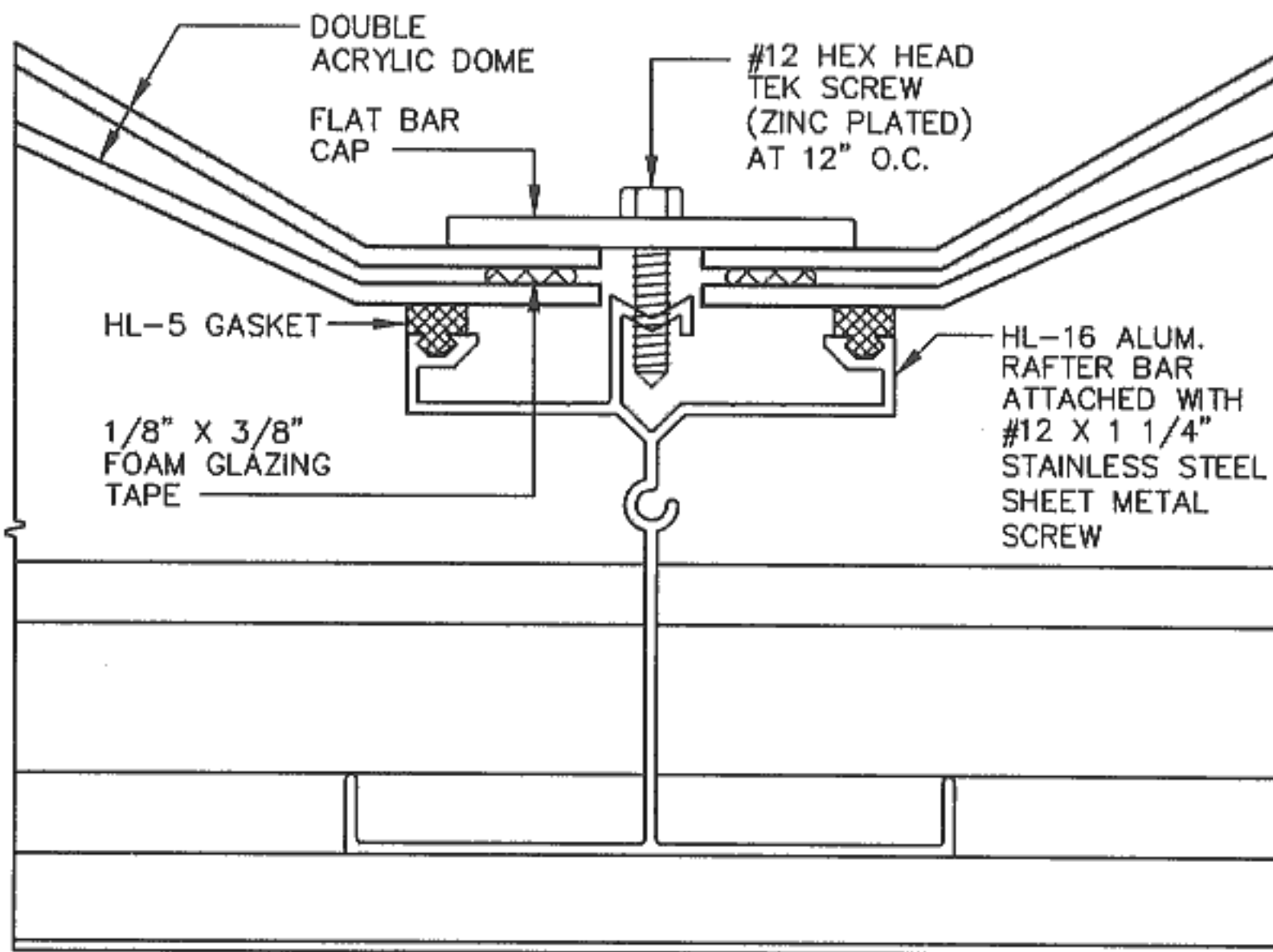
② TYPICAL RAFTER 1/2 FULL SCALE
