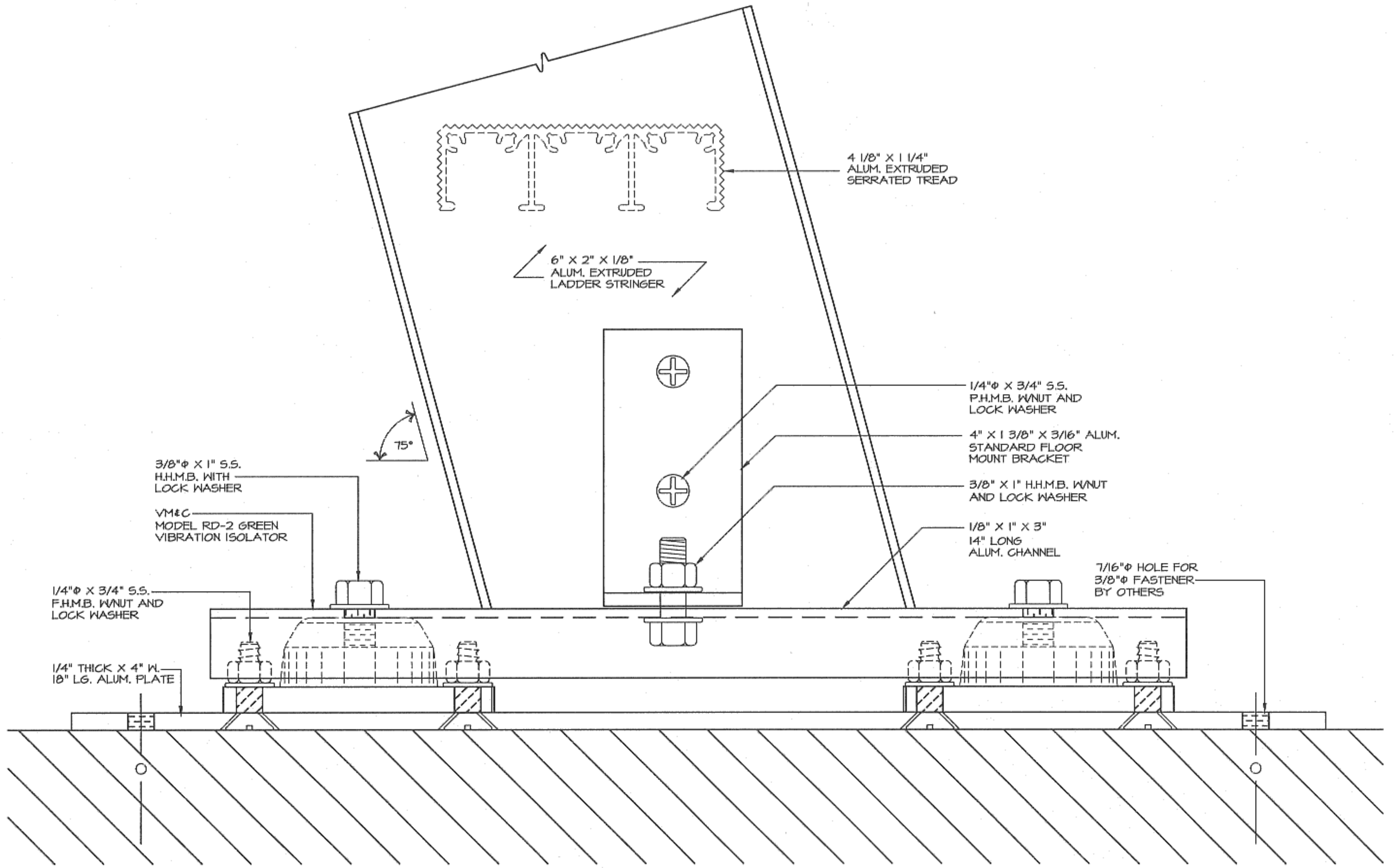
SEISMIC MOUNTING BRACKET SIDE VIEW (OPTIONAL) 1/2 FULL SCALE
