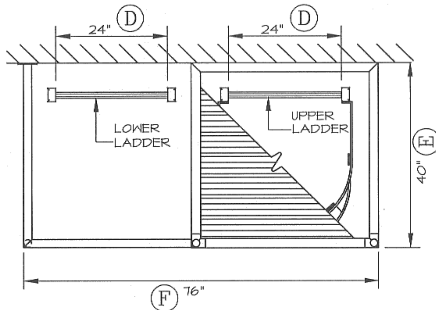
A PLATFORM PLAN 3/8" = 1' - 0"
